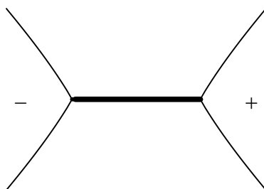
Fig. 1. d = 2, \ell = 1 .
