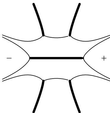
Fig. 8. d = 6, \ell = 3 .
