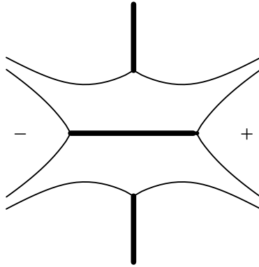
Fig. 4. d = 4, \ell = 2 .
