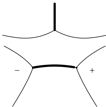
Fig. 2. d = 3, \ell = 1 .
