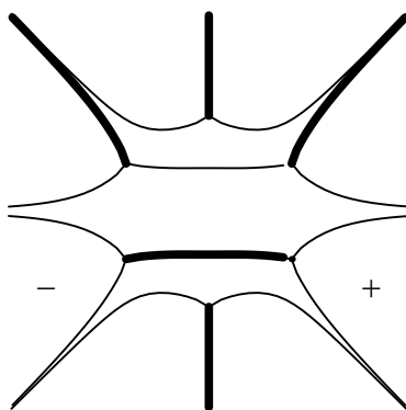
Fig. 7. d = 6, \ell = 2 .
