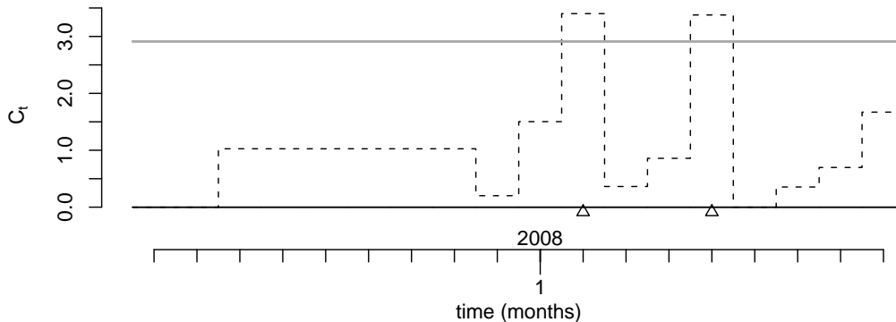
Figure 8: CUSUM statistic C_t for the pediatricist data together with the threshold h = 2.911 . Triangles indicate detected change-points.
