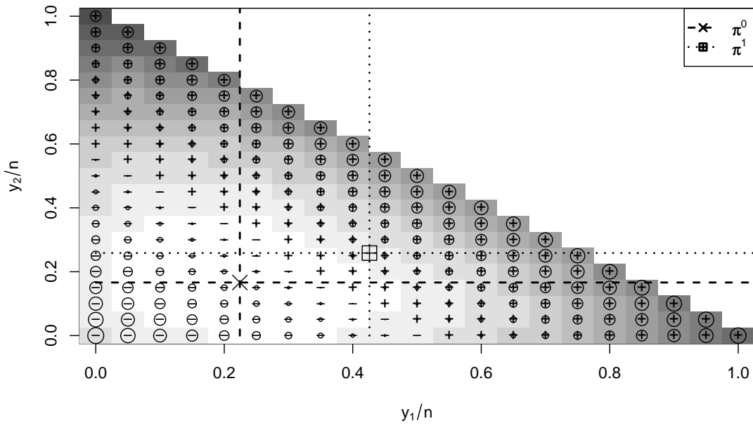
Figure 2: Illustration of the LLR for a M_3(20, \boldsymbol{\pi}) multinomial CUSUM with \boldsymbol{\pi}^0 = (0.22, 0.17, 0.61)' and \boldsymbol{\pi}^1 = (0.43, 0.26, 0.32)' . Shown are the first two components y_1 and y_2 of each possible state \mathbf{y} . Circle sizes indicate magnitude and \pm the sign of the LLR. Also shown are the in-control and out-of-control probabilities. Shading indicates the probability of \mathbf{y} in a model with \boldsymbol{\pi} = \boldsymbol{\pi}^0 – the whiter the cell the higher is the probability of the corresponding state.
