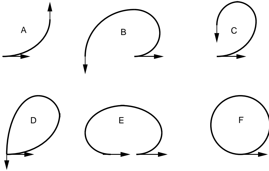
Fig.2. Types of (non)strictly disconjugate curves on \mathbb{S}^2 (all cases except A are nonstrictly disconjugate).
