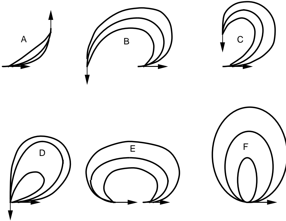
Fig.3. Disconjugate curves form a connected set for all arrangements of initial and final flags.
