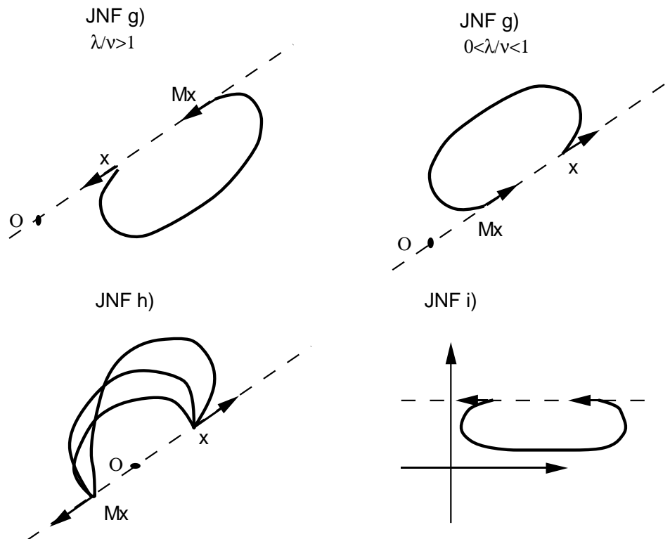
Fig.10. Special flags and their discojugate curves for JNF g), h) and i).
