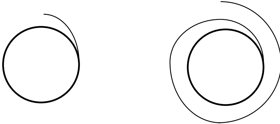
Fig. 5. Illustration of the covering homotopy property.
