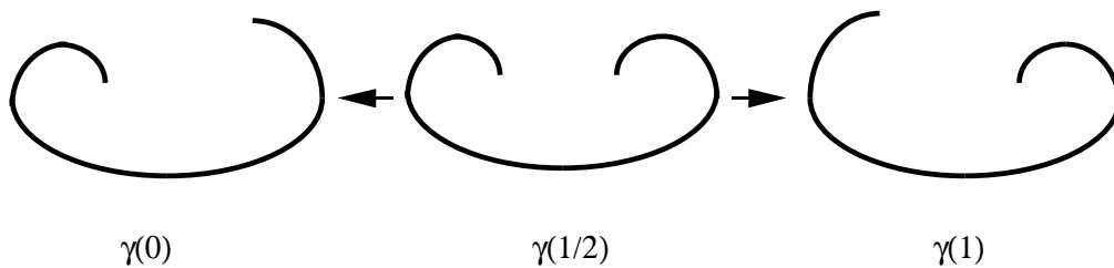
Fig. 5. Illustration of the covering homotopy property.
