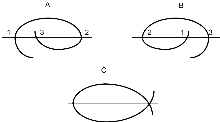
Fig.4. 3 possible forms of simplest conjugate fragments.
